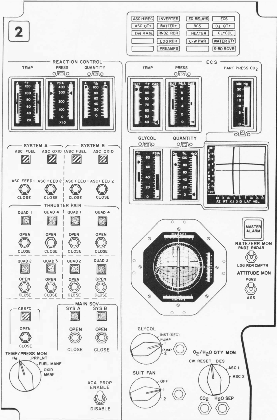
Figure 3.3. Center Console, Systems Engineer (Panel 2)
