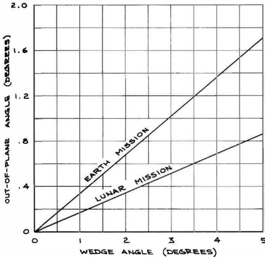
Figure 26.1. Out-of-Plane Angle at Switchover to Node at Rendezvous Versus Wedge Angle for Lunar and Earth Mission
