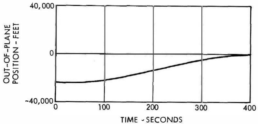
Figure 22.4. Out-of-Plane Position versus Time for Lunar Surface Abort
