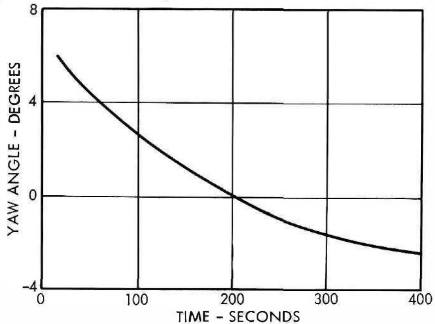
Figure 22.7. Yaw Angle versus Time for Lunar Surface Abort
