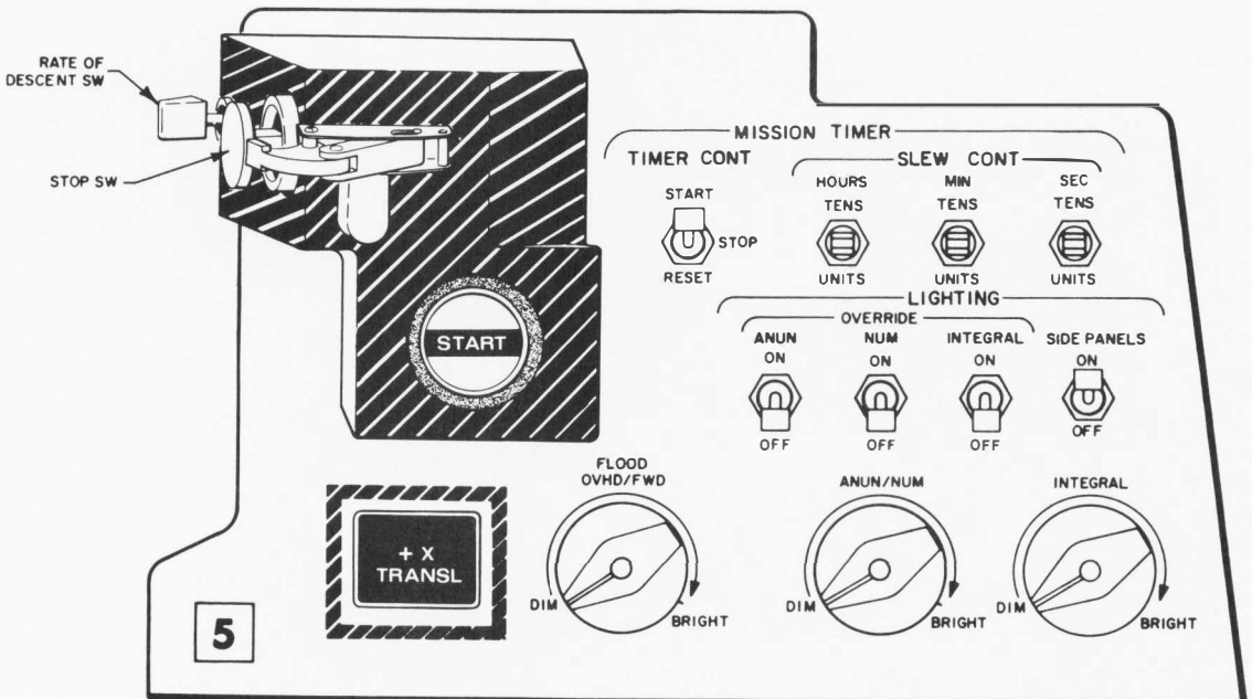
Figure 3.5. Bottom Panel (Panel 5)
