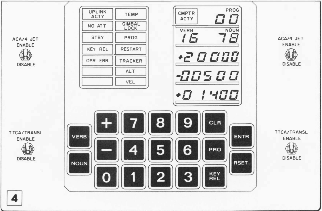
Figure 3.6. Bottom Center Panel (DSKY) (Panel 4)
