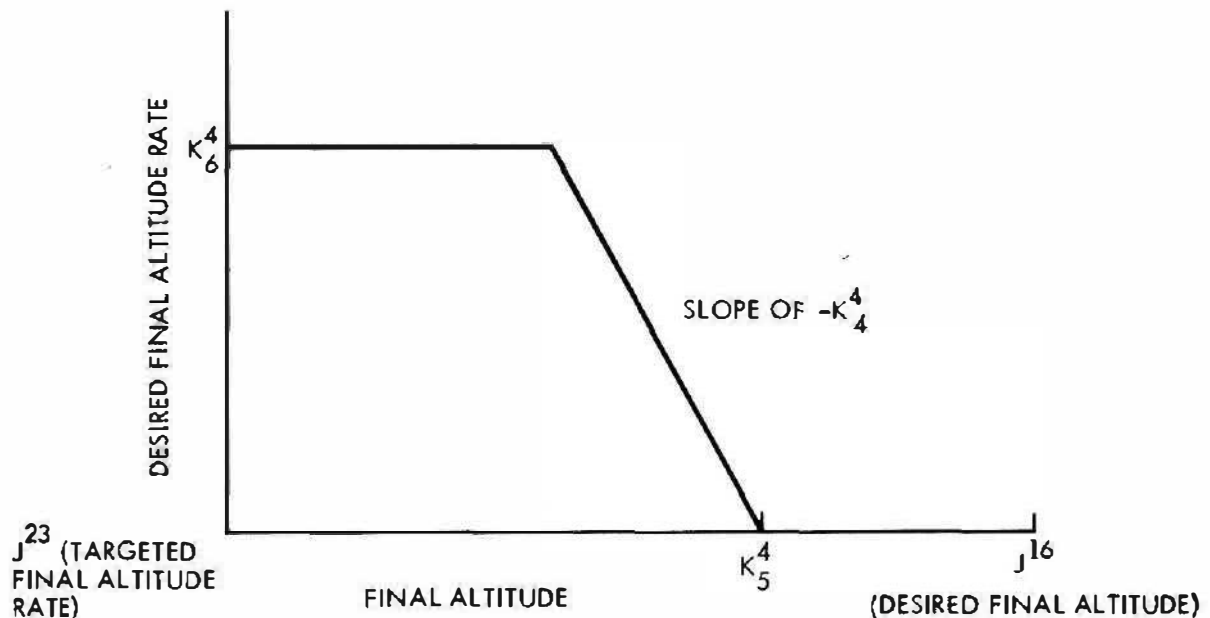
Figure 22.1. Desired Final Altitude Rate versus Final Altitude
