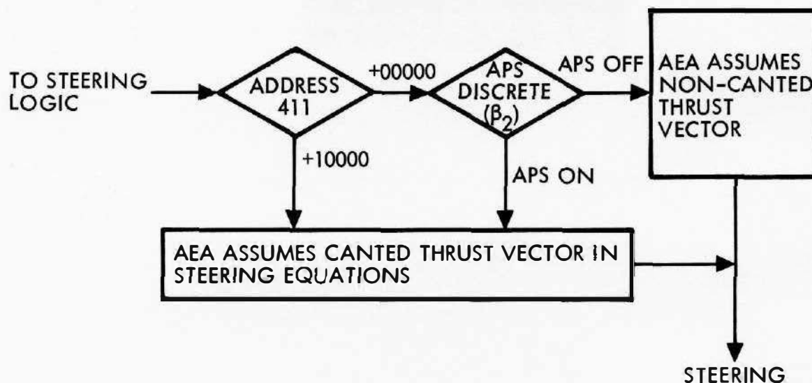
Figure 20.1. Canted Thrust Selection Logic
